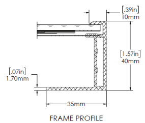
FRAME PROFILE
